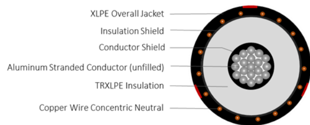
SERIES U15ATX
