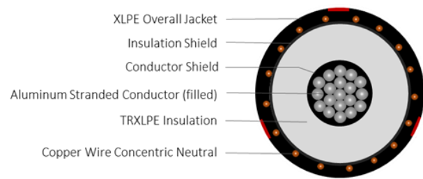
SERIES U25SATX
